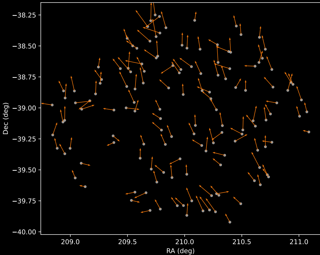
GALAH DR4 Cluster 2 Proper Motion Vectors (n=142)
