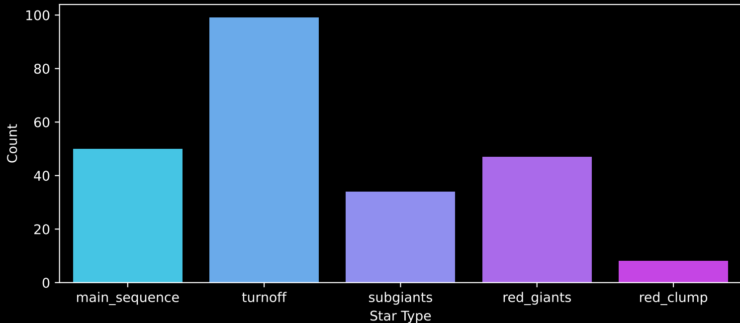
GALAH DR4 Field: [3886] Count plot of Star Type
