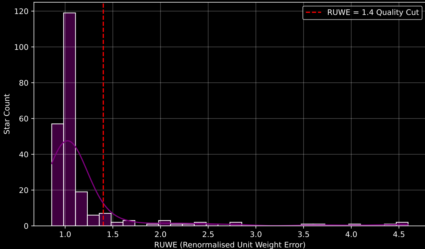
GALAH DR4 Field [3886] RUWE Distribution (n= 230)
