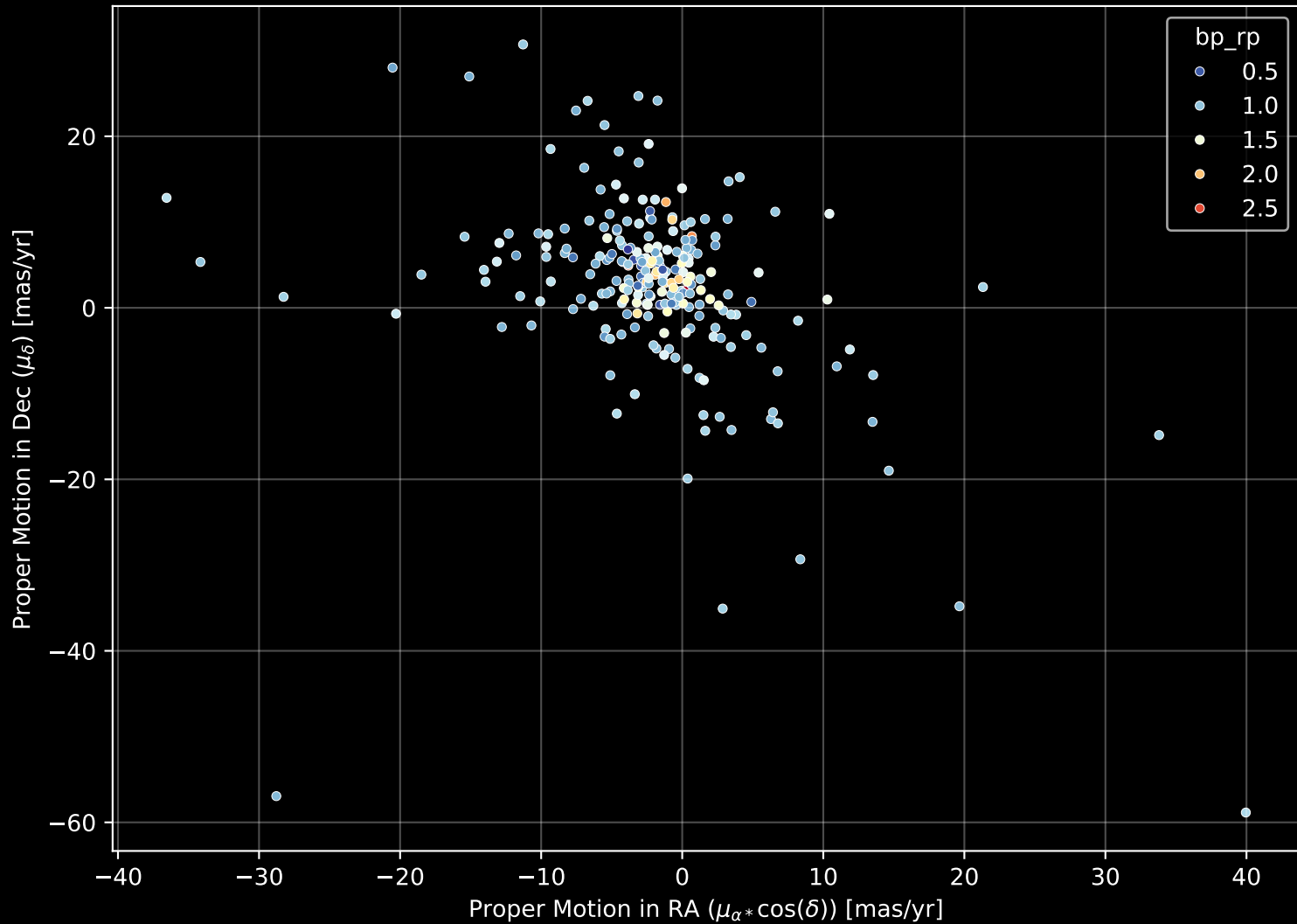
GALAH DR4 Field: [3886] Proper Motion Diagram (n= 238)
